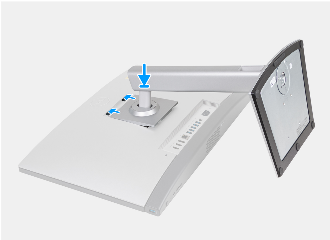
Figure 20. Installing the Height Adjustable Stand (HAS)
