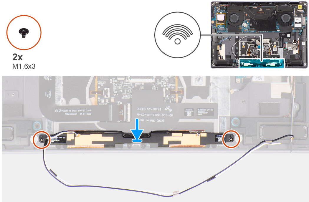
Figure 38. Installing the WLAN antenna module
