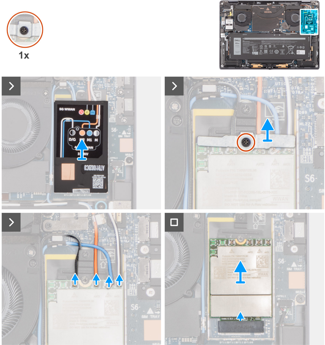
Figure 27. Removing the WWAN card
