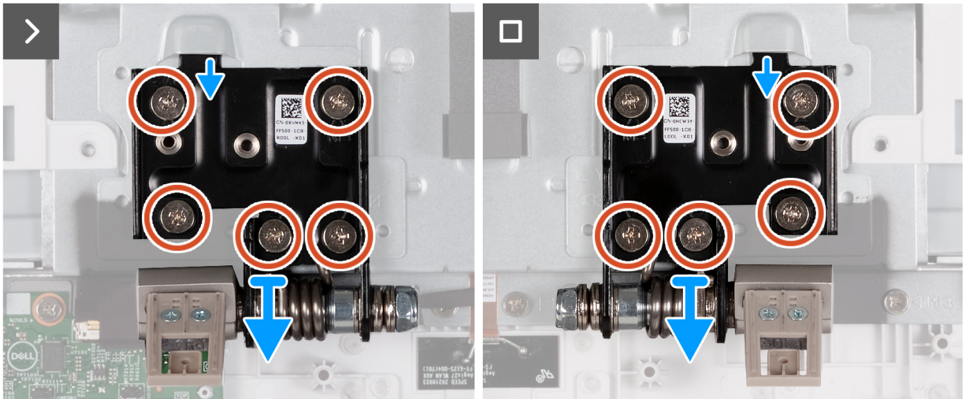
Figure 24. Removing the stand hinges
