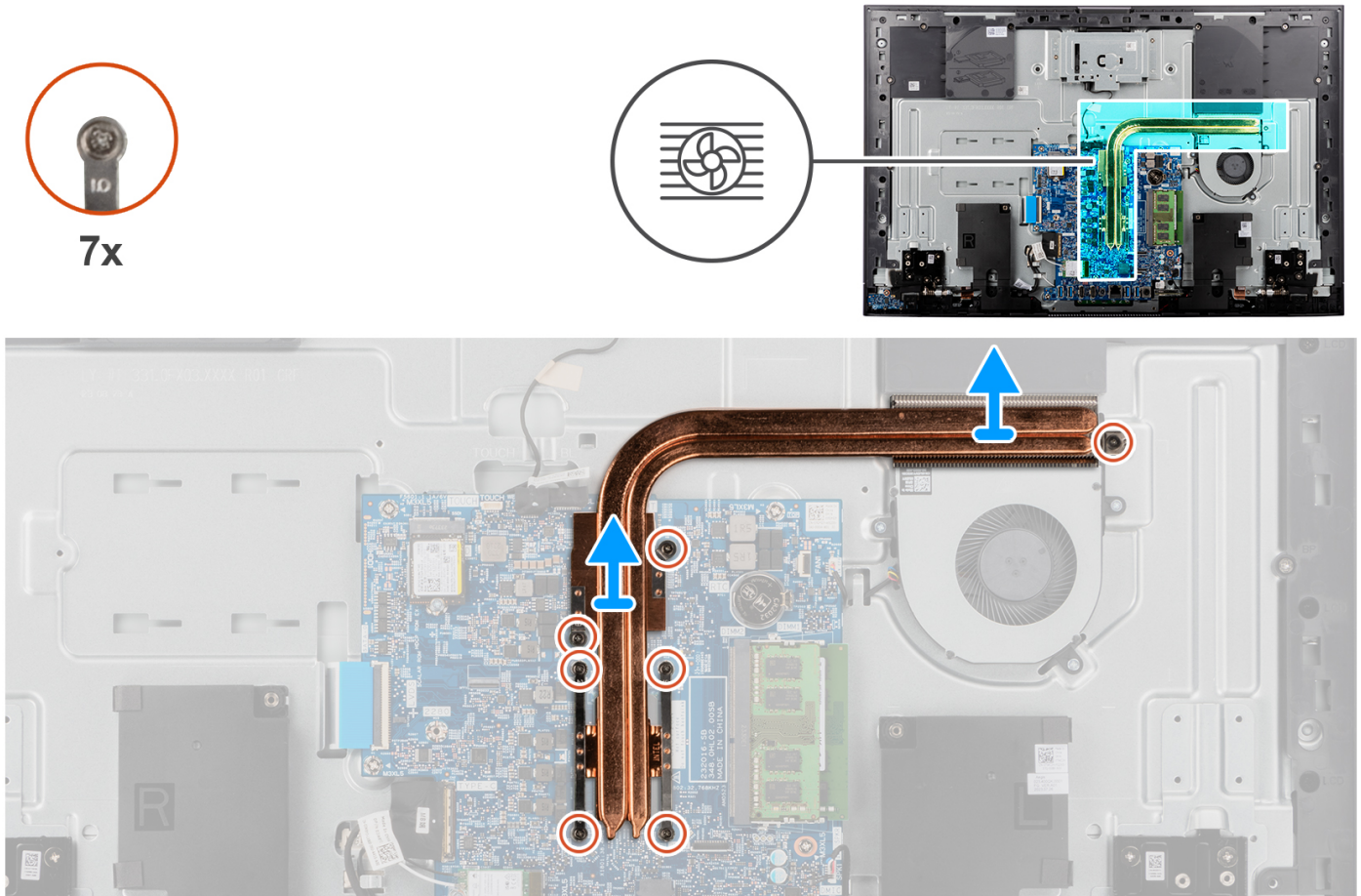
Figure 44. Removing the heat sink- discrete
