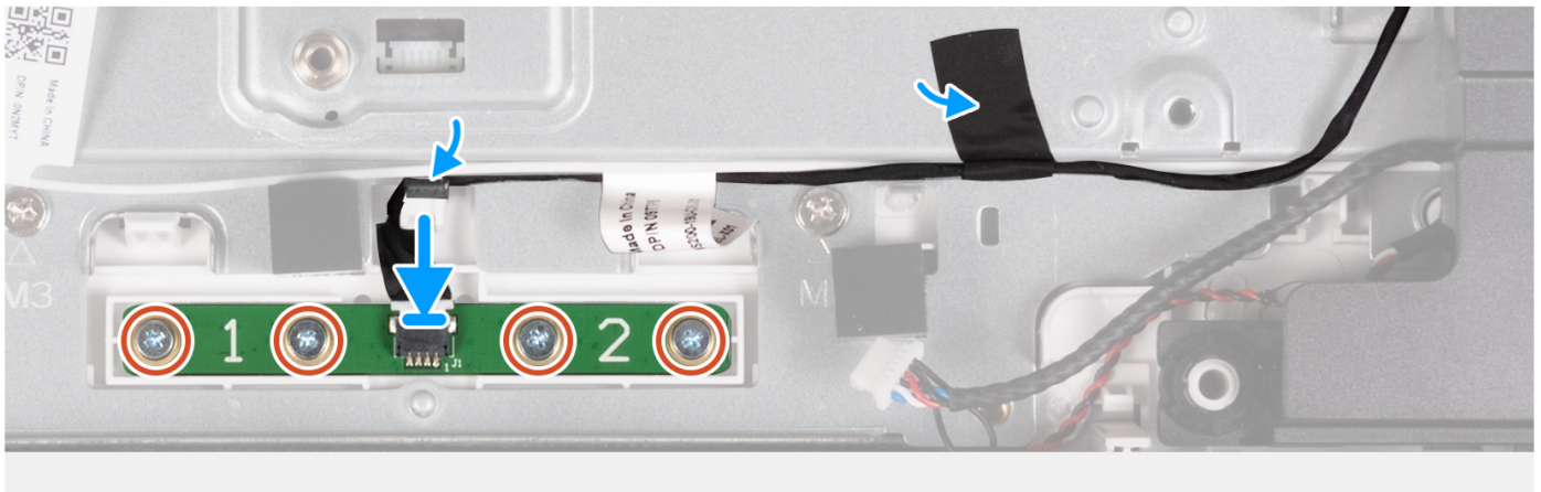
Figure 57. Installing the microphones
