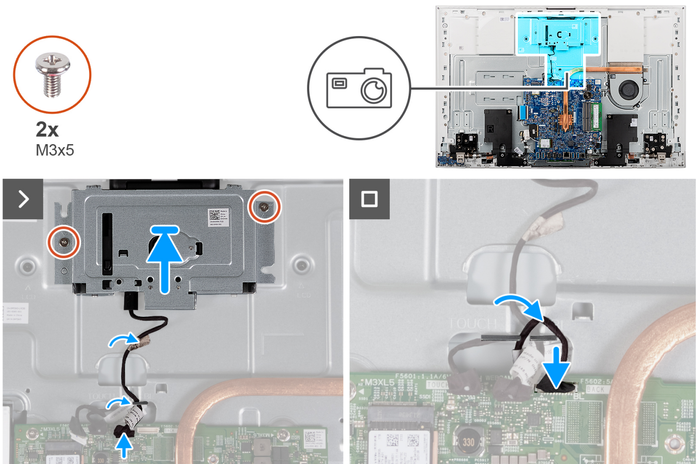
Figure 35. Installing the camera
