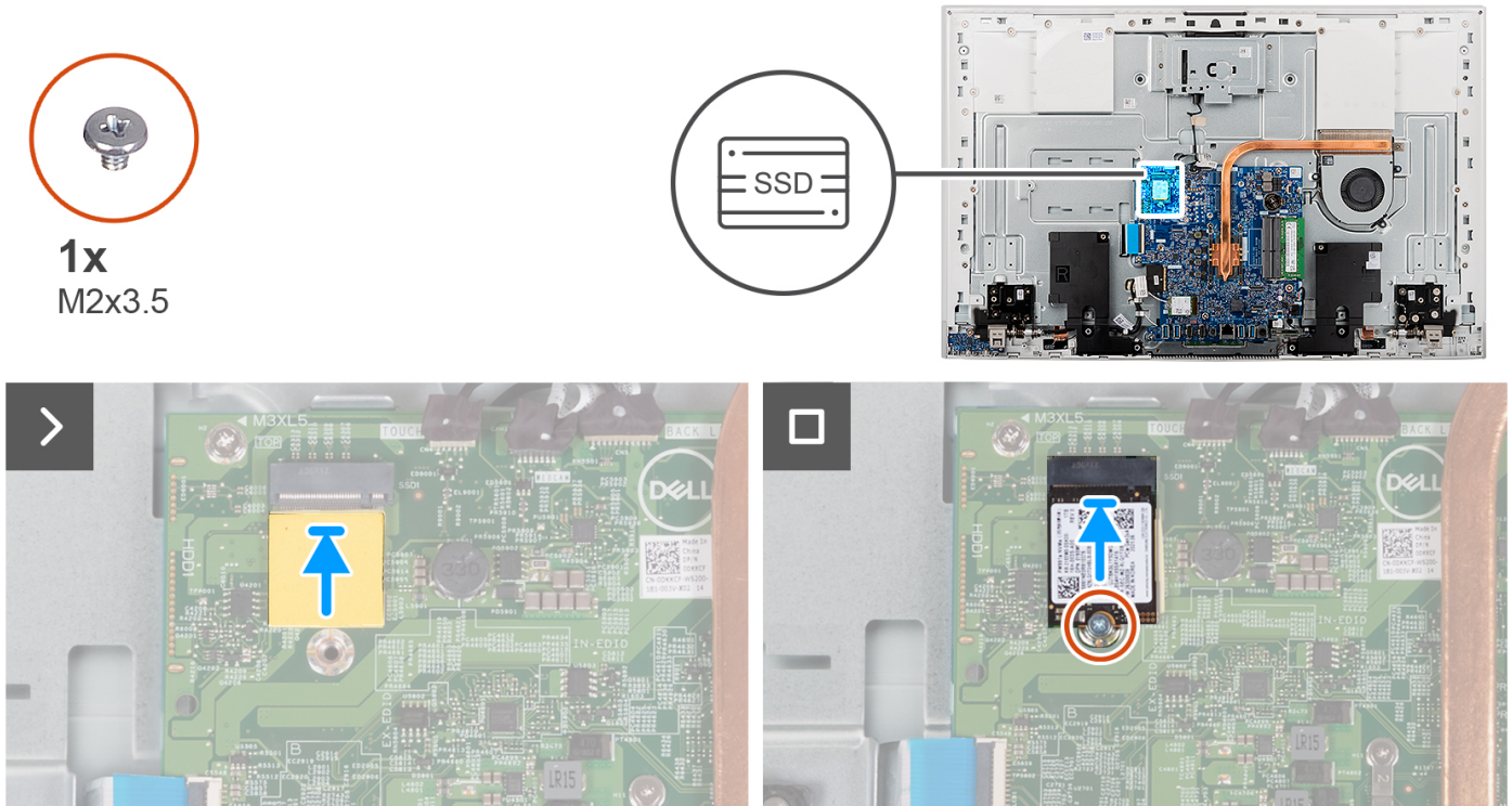
Figure 29. Installing the M.2 2230 solid-state drive
