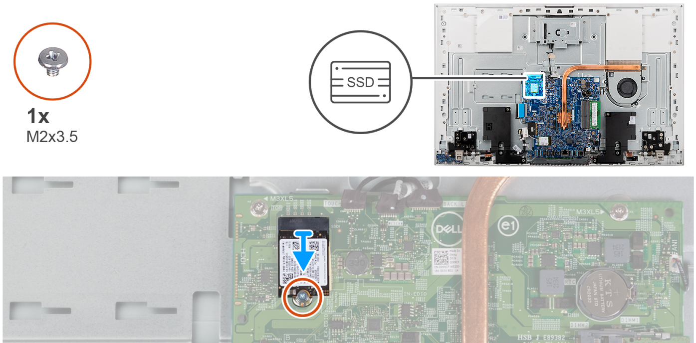
Figure 28. Removing the M.2 2230 solid-state drive
