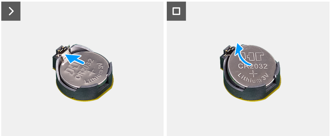
Figure 40. Removing the coin-cell battery
