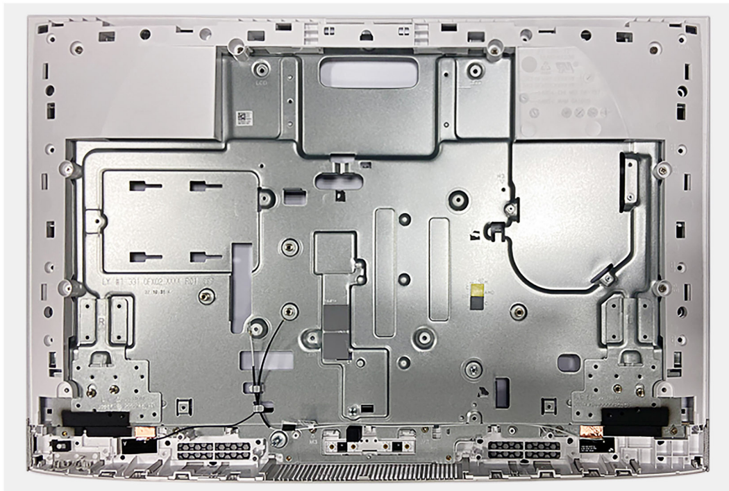
Figure 64. Removing the middle-frame assembly
