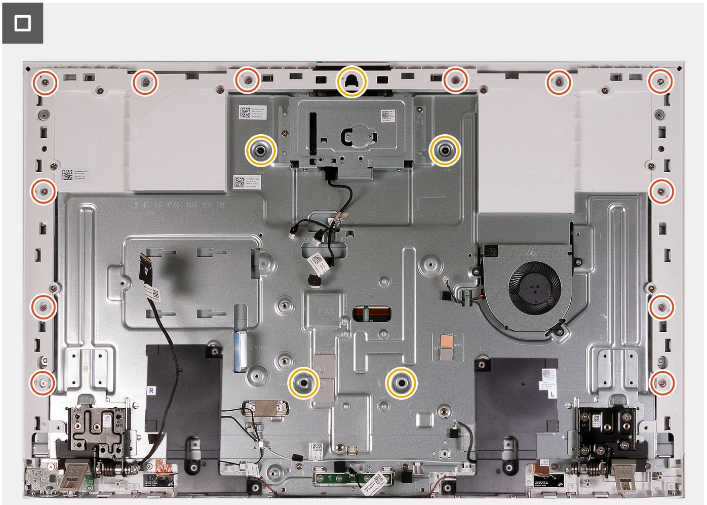
Figure 63. Replacing the screws
