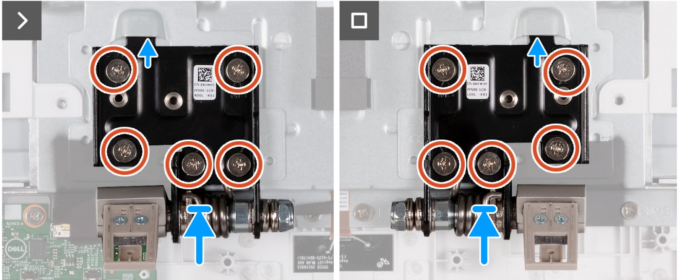
Figure 25. Installing the stand hinges
