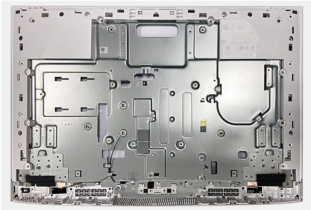
Figure 65. Installing the middle-frame assembly
