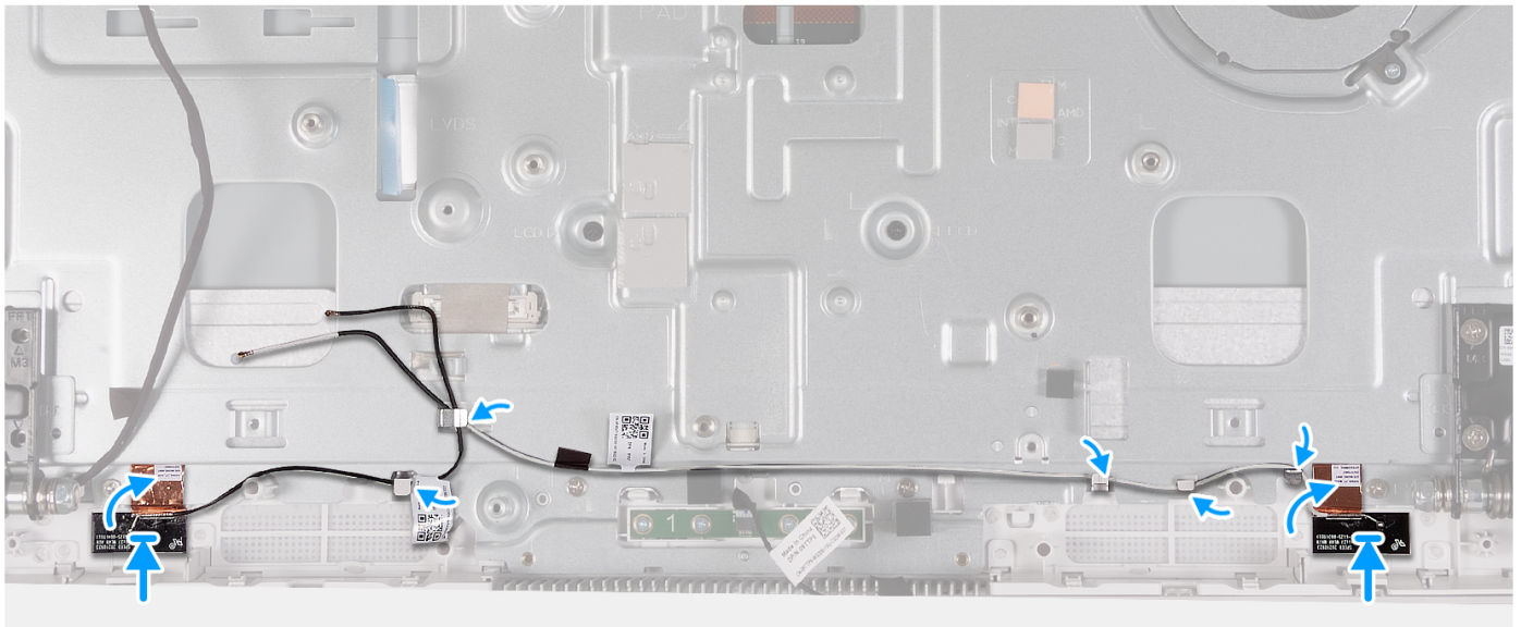
Figure 59. Installing the antennas
