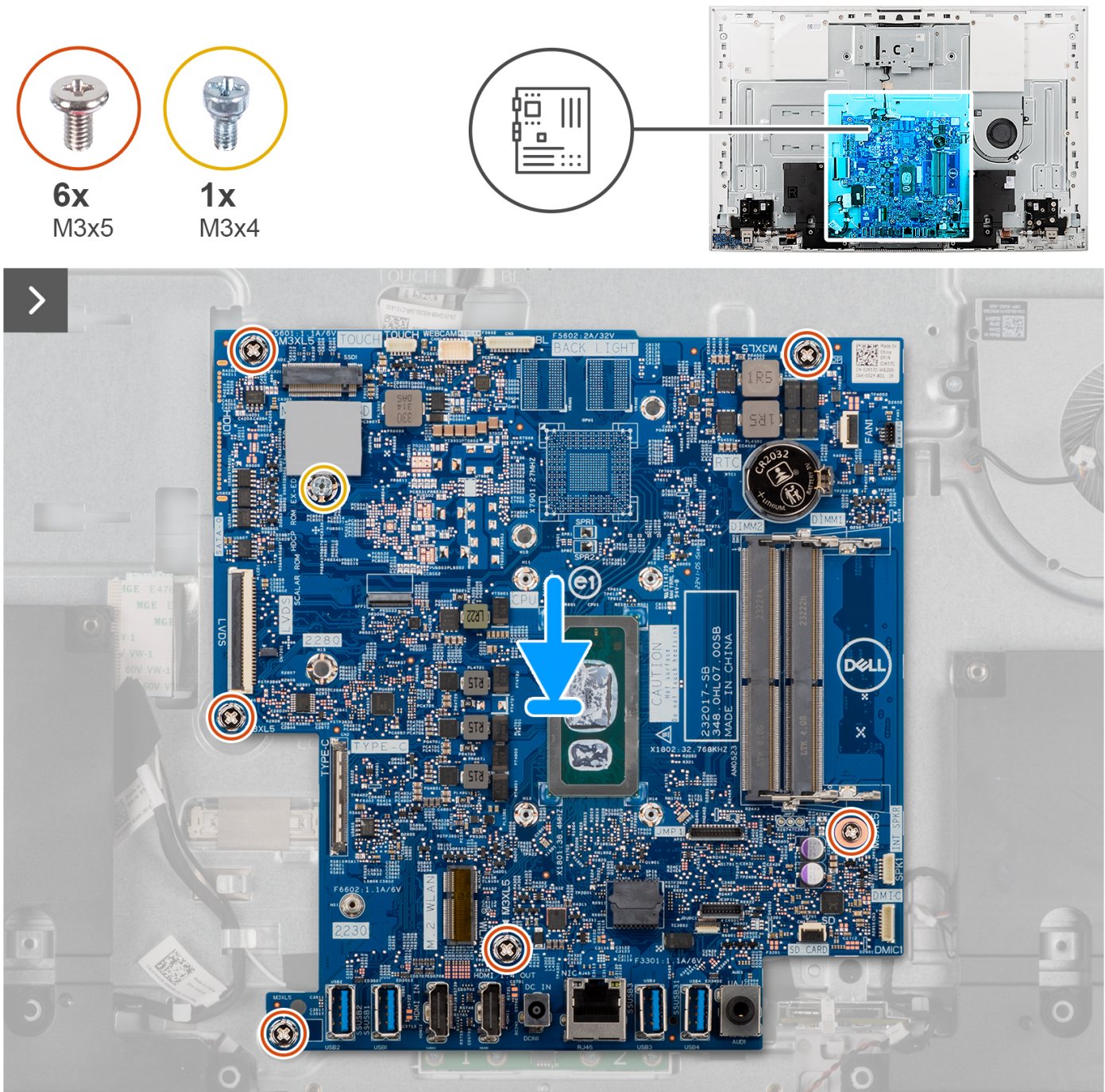
Figure 54. Placing the system board in the chassis
