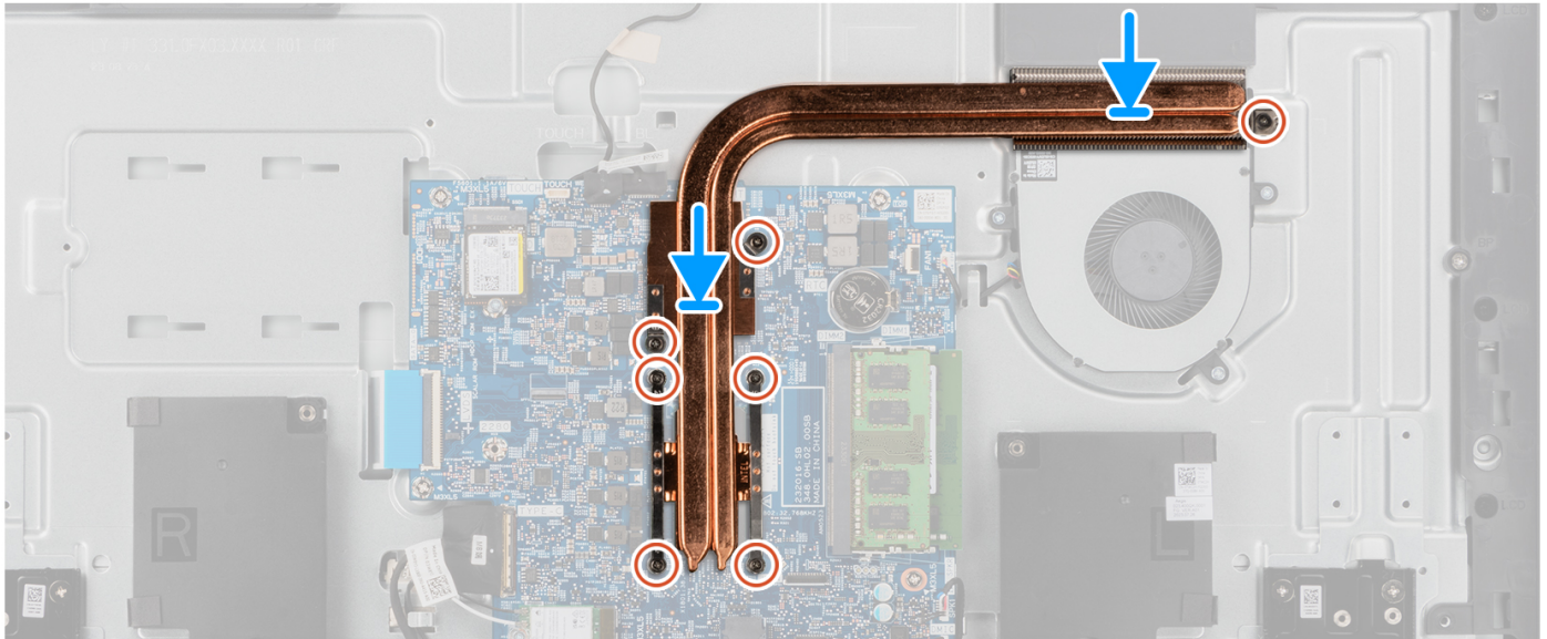
Figure 45. Installing the heat sink- discrete
