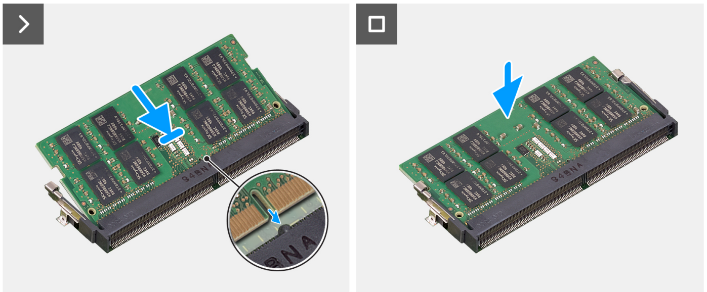
Figure 31. Installing the memory module
