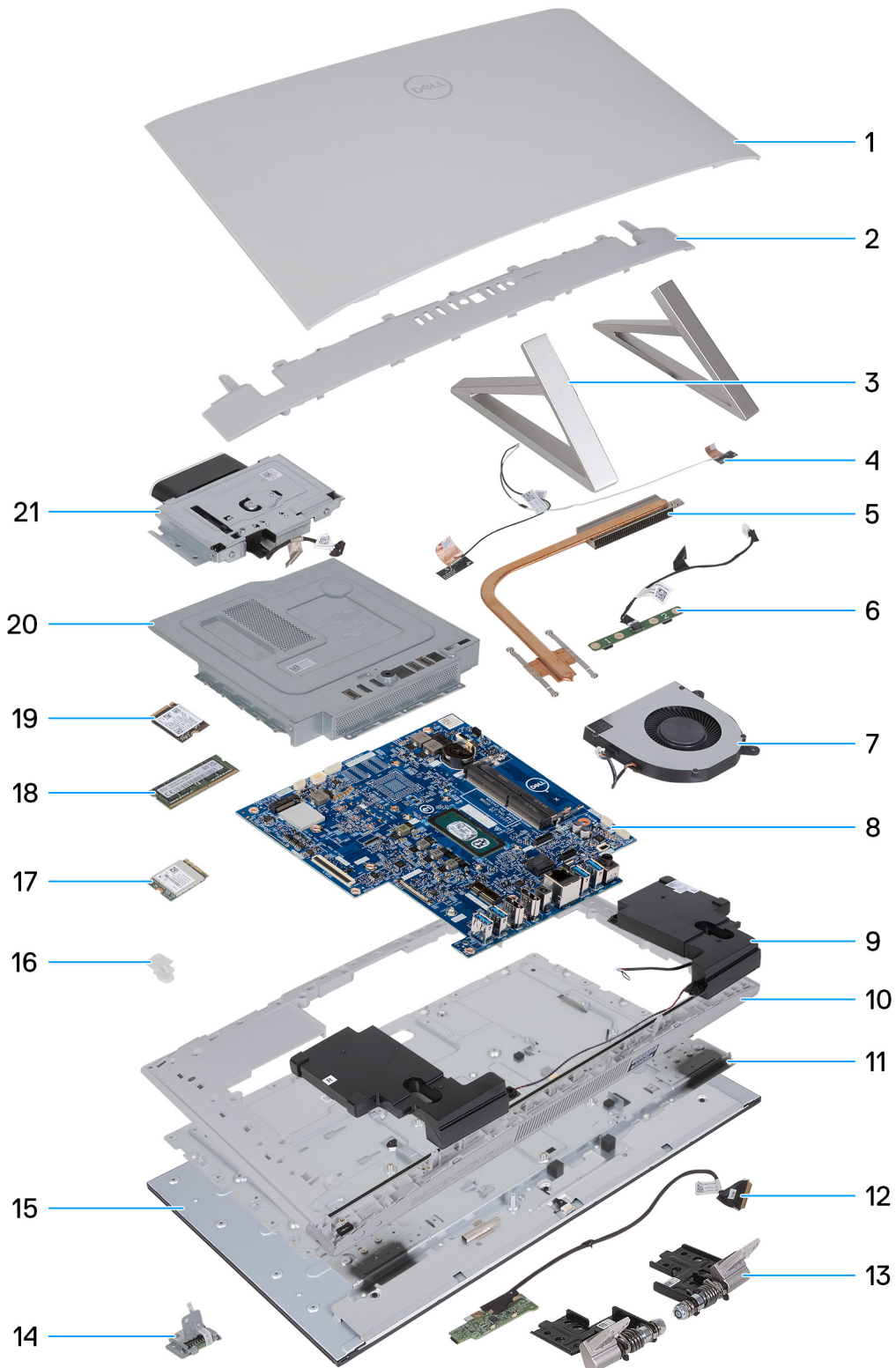
Figure 15. Major components of your computer
