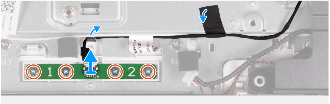
Figure 56. Removing the microphones
