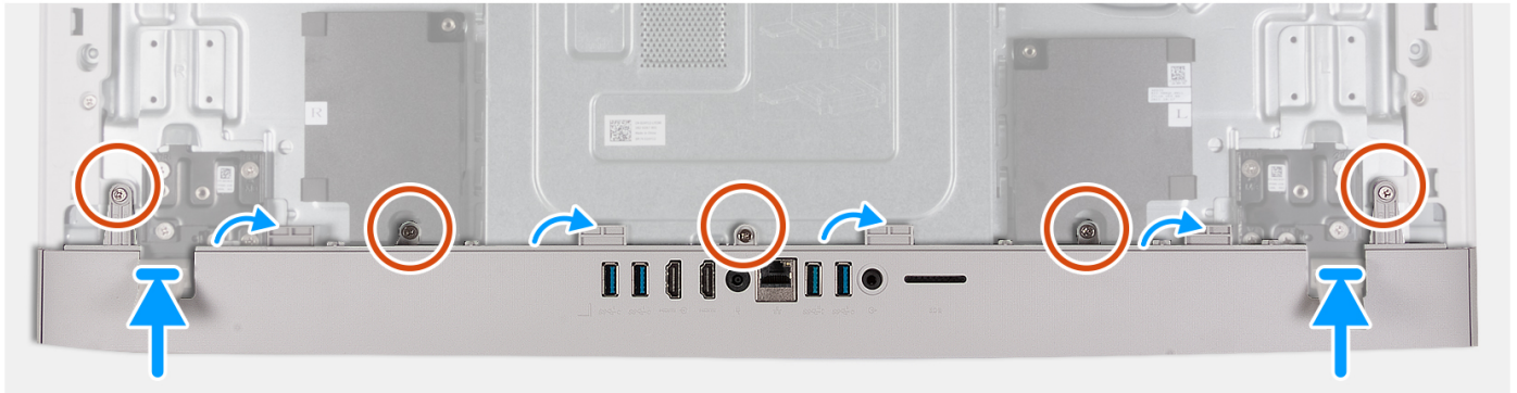
Figure 23. Installing bottom cover
