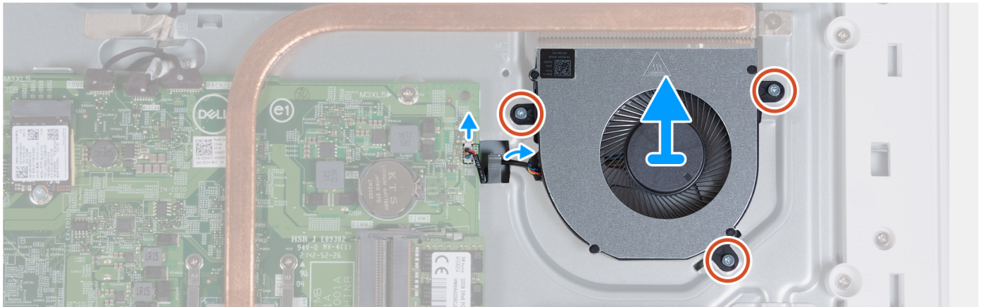
Figure 36. Removing the fan
