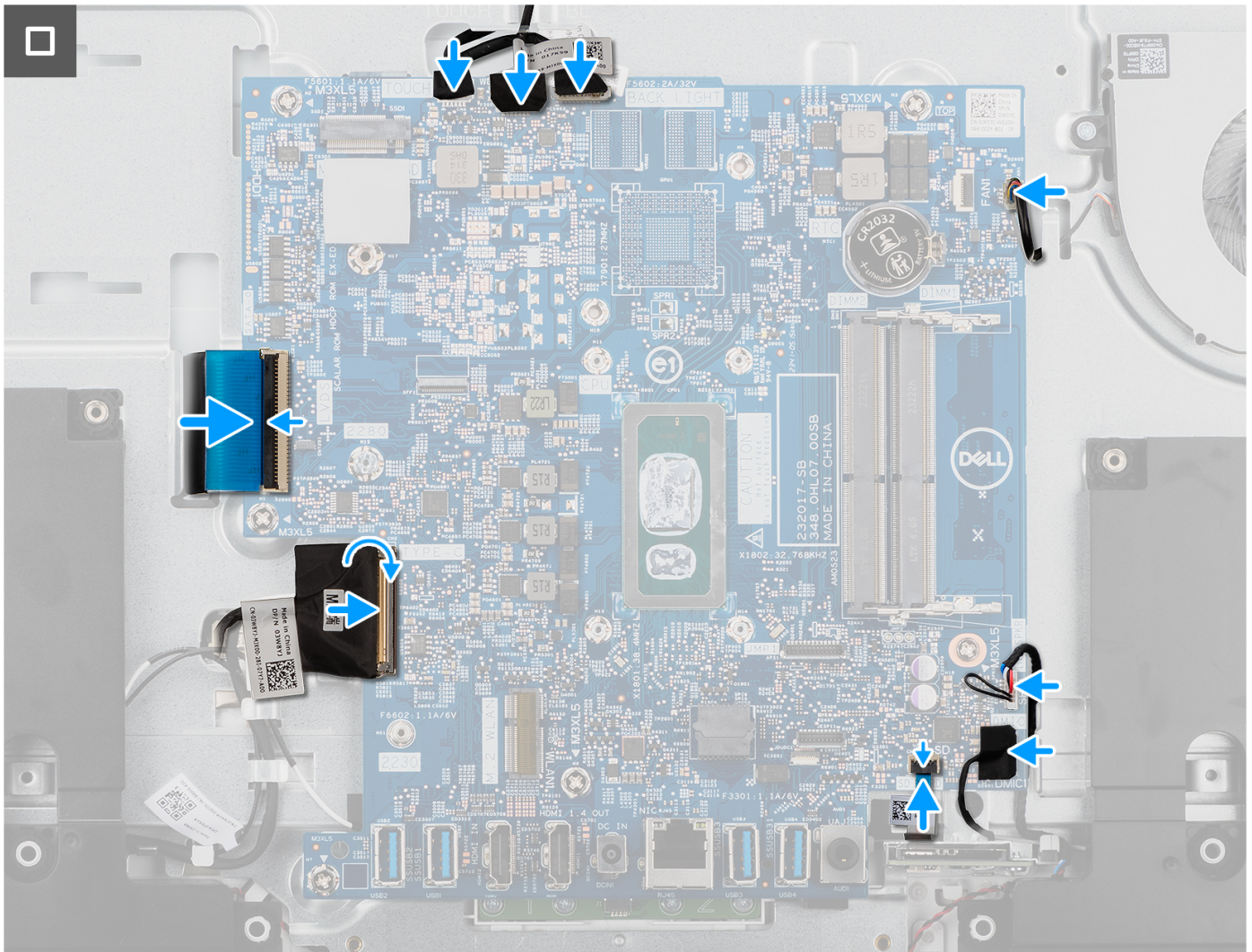
Figure 55. Installing the system board
