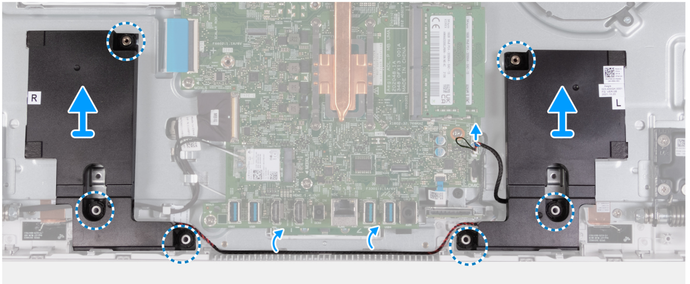
Figure 38. Removing the speakers
