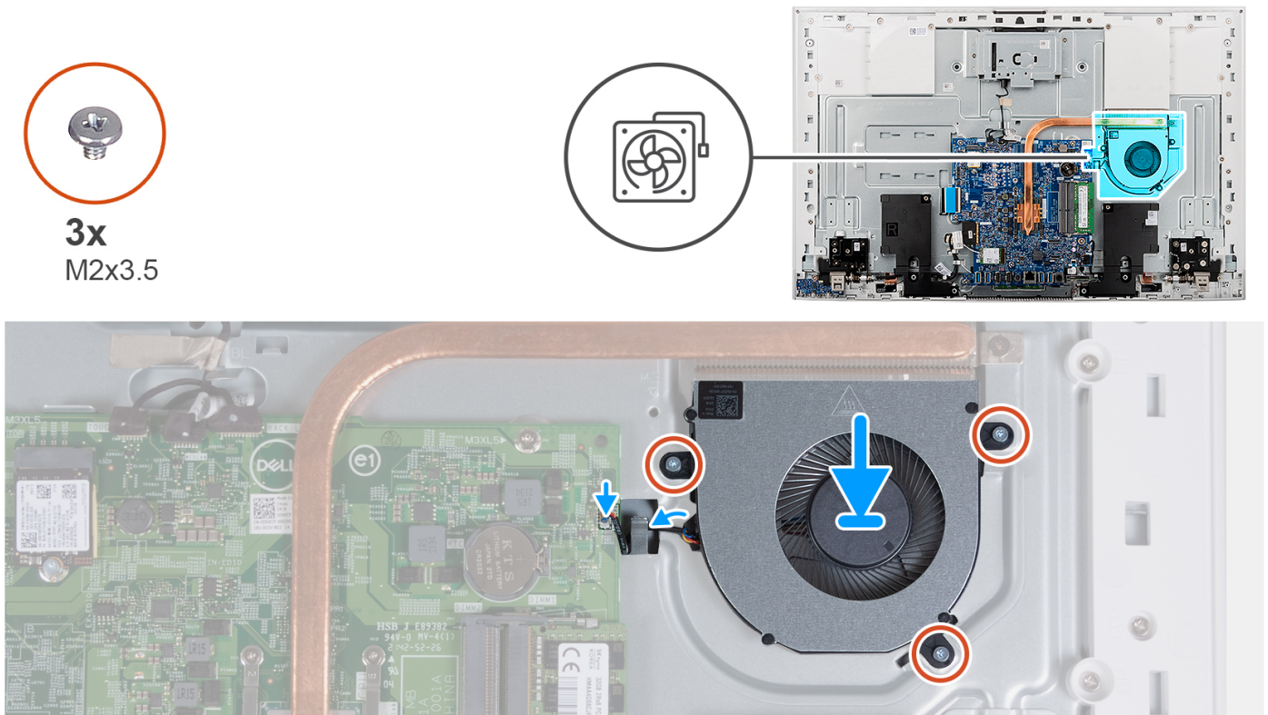
Figure 37. Installing the fan
