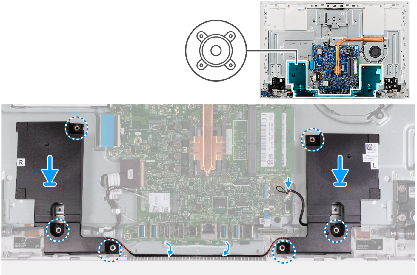
Figure 39. Installing the speakers
