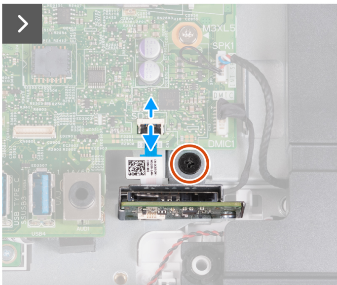
Figure 46. Removing the media-card reader
