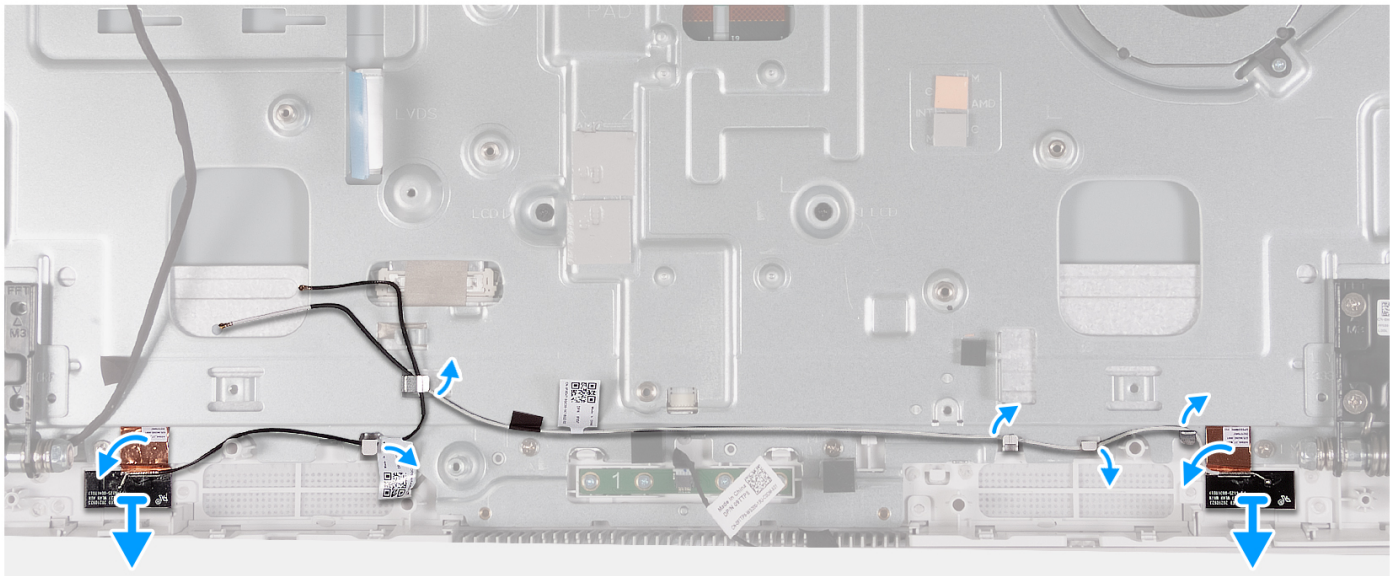
Figure 58. Removing the antennas
