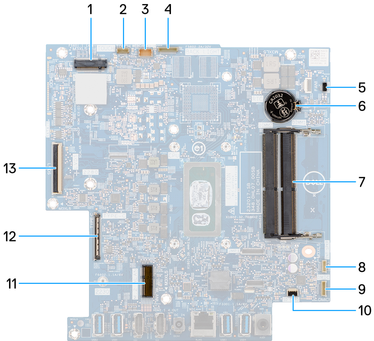
Figure 50. System-board connectors
