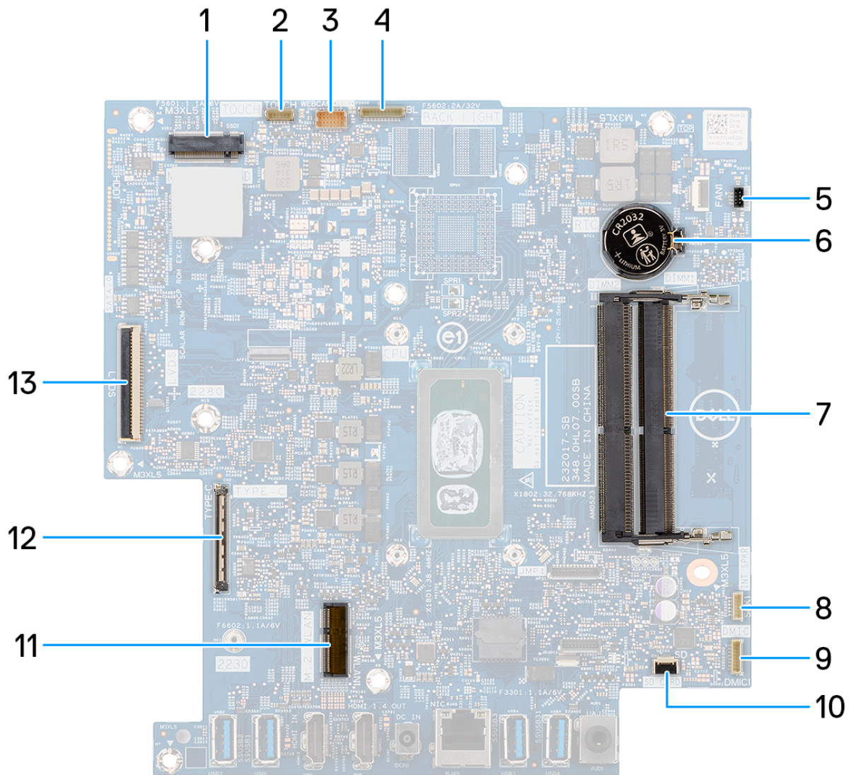
Figure 53. System-board connectors
