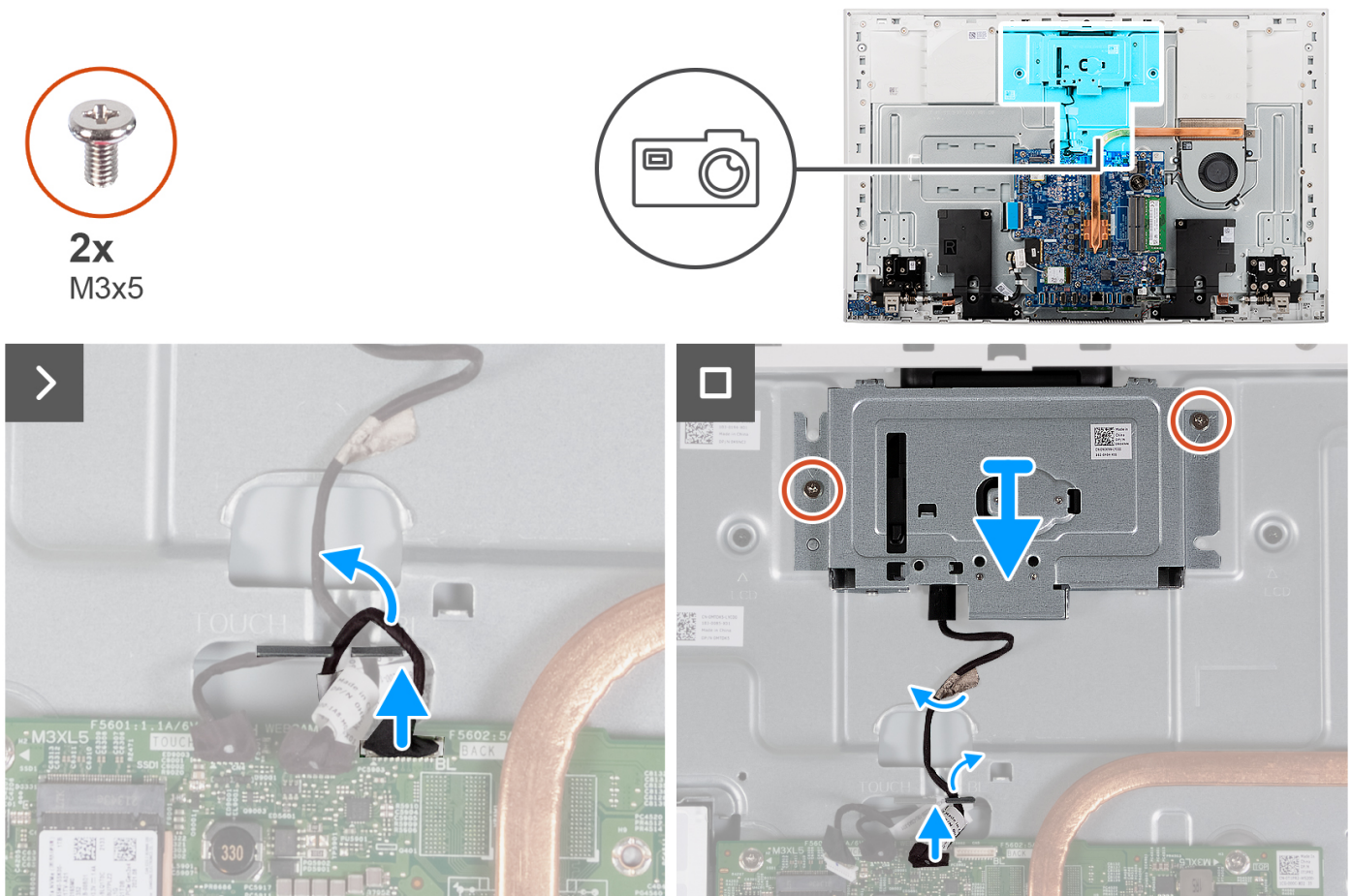
Figure 34. Removing the camera
