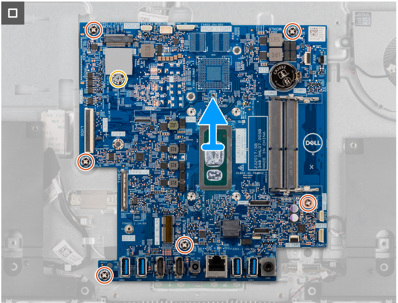
Figure 52. Lifting the system board off the chassis
