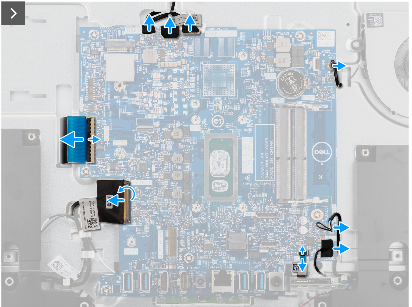
Figure 51. Removing the system board
