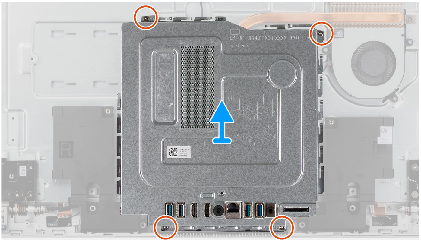
Figure 26. Removing the system-board shield
