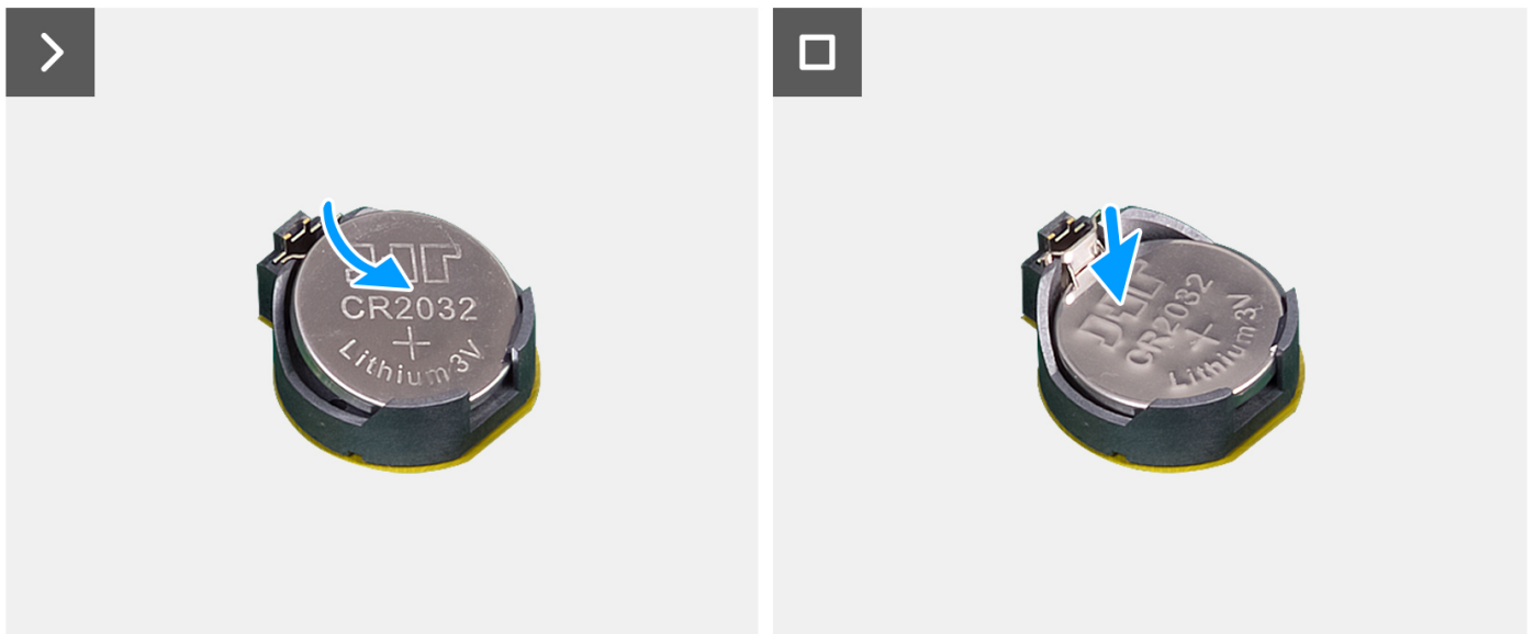
Figure 41. Installing the coin-cell battery
