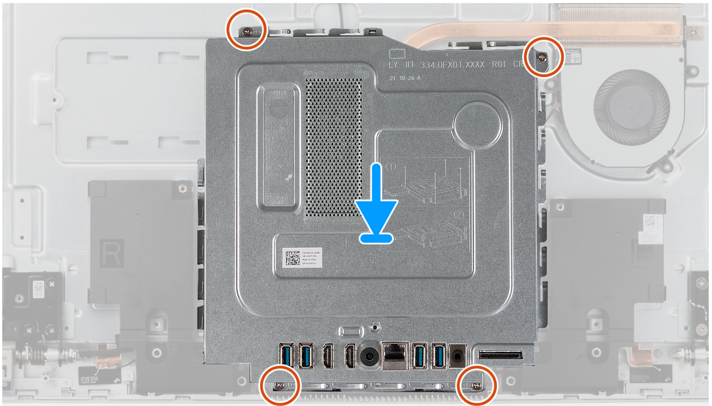
Figure 27. Installing the system-board shield
