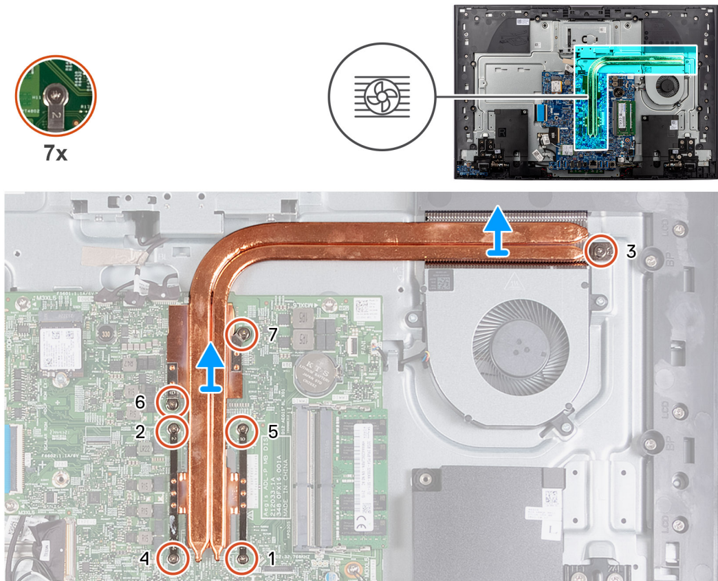
Figure 44. Removing the heat sink- discrete
