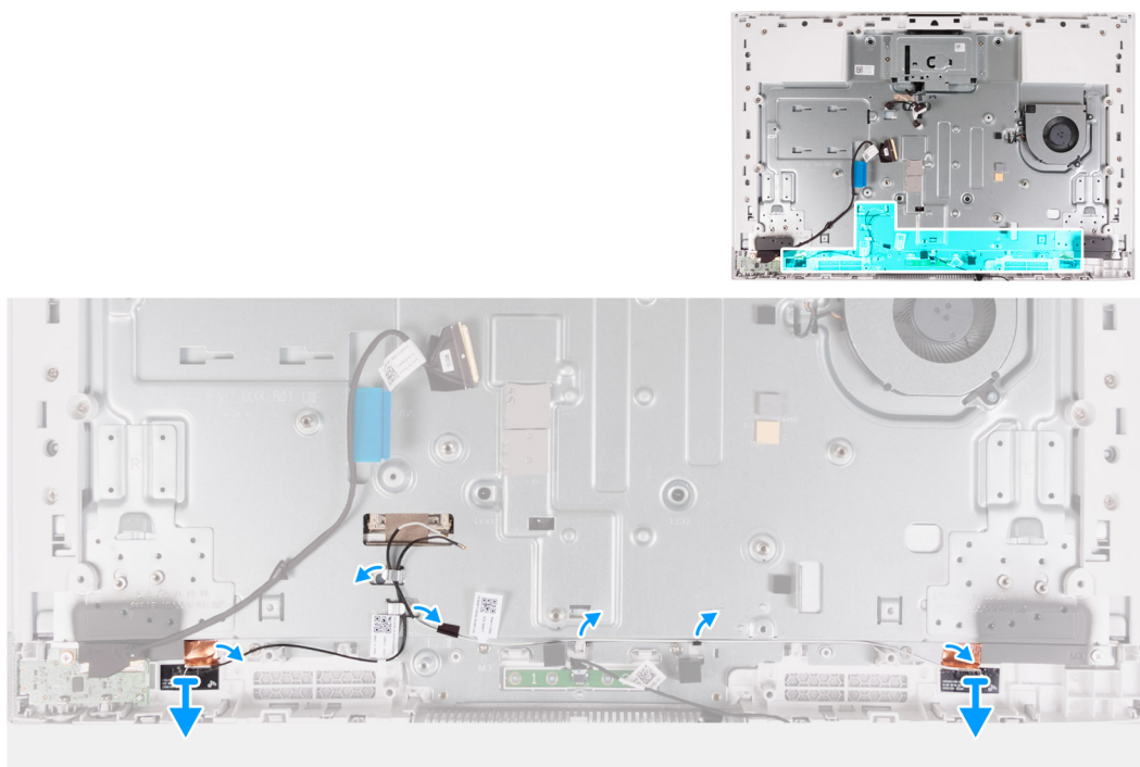
Figure 58. Removing the antennas
