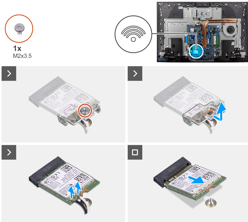
Figure 32. Removing the wireless card
