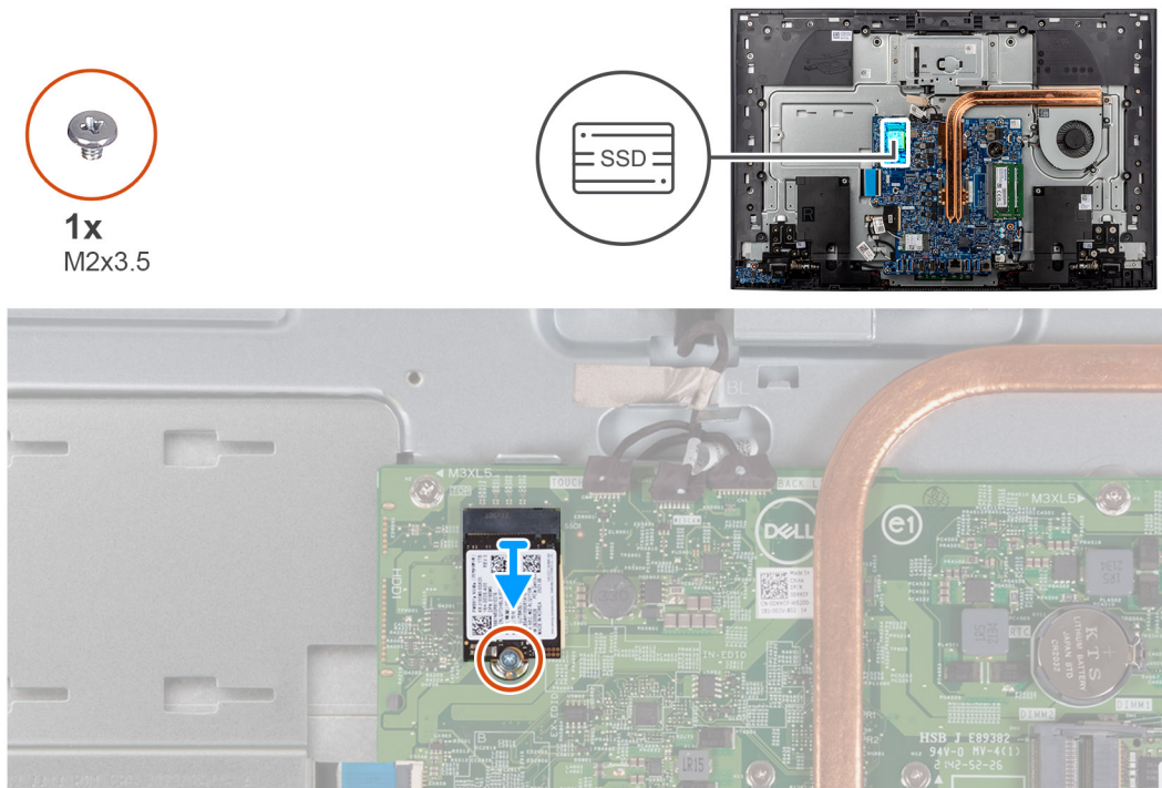
Figure 28. Removing the M.2 2230 solid-state drive
