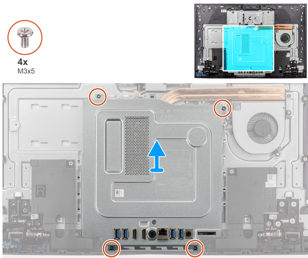
Figure 26. Removing the system-board shield
