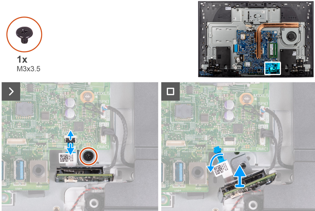
Figure 46. Removing the media-card reader
