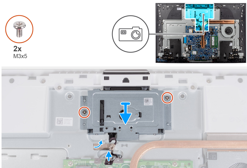
Figure 34. Removing the camera
