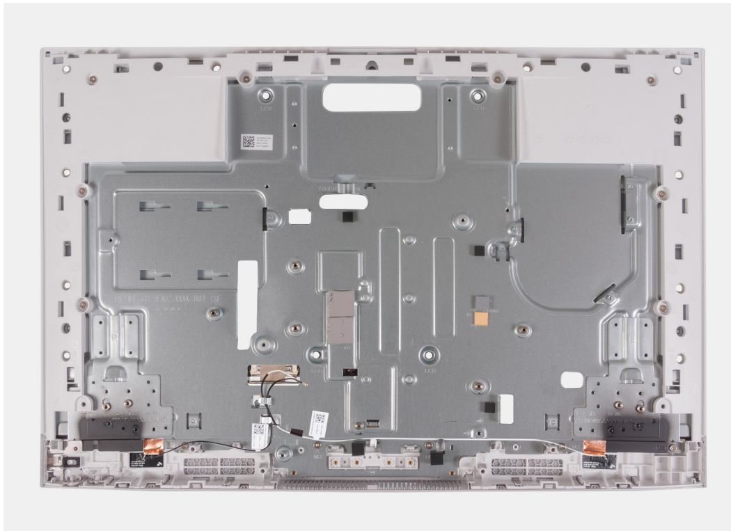
Figure 65. Installing the middle-frame assembly
