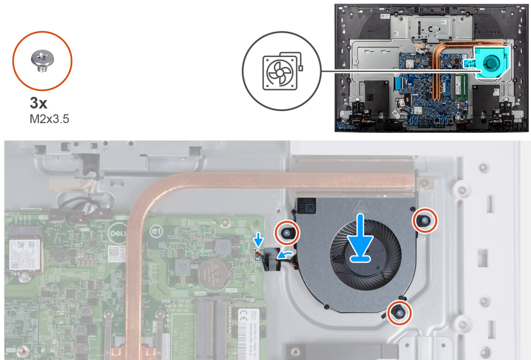
Figure 37. Installing the fan
