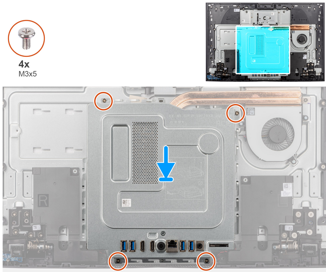
Figure 27. Installing the system-board shield
