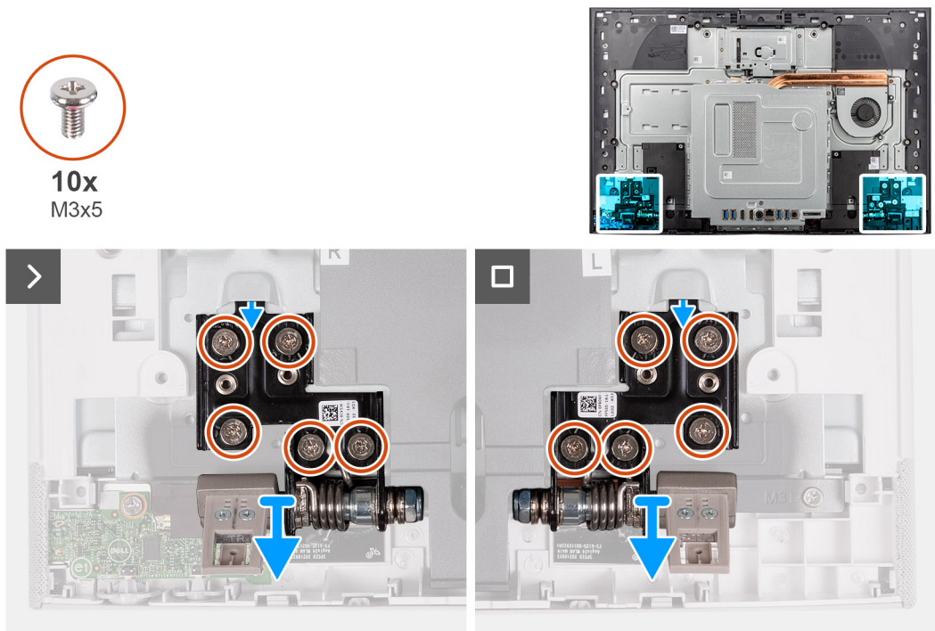
Figure 24. Removing the stand hinges
