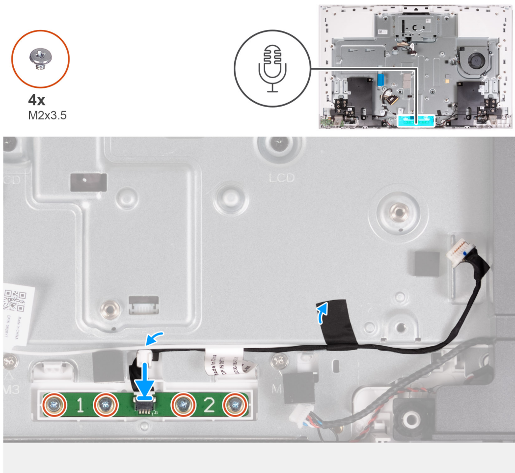
Figure 57. Installing the microphones
