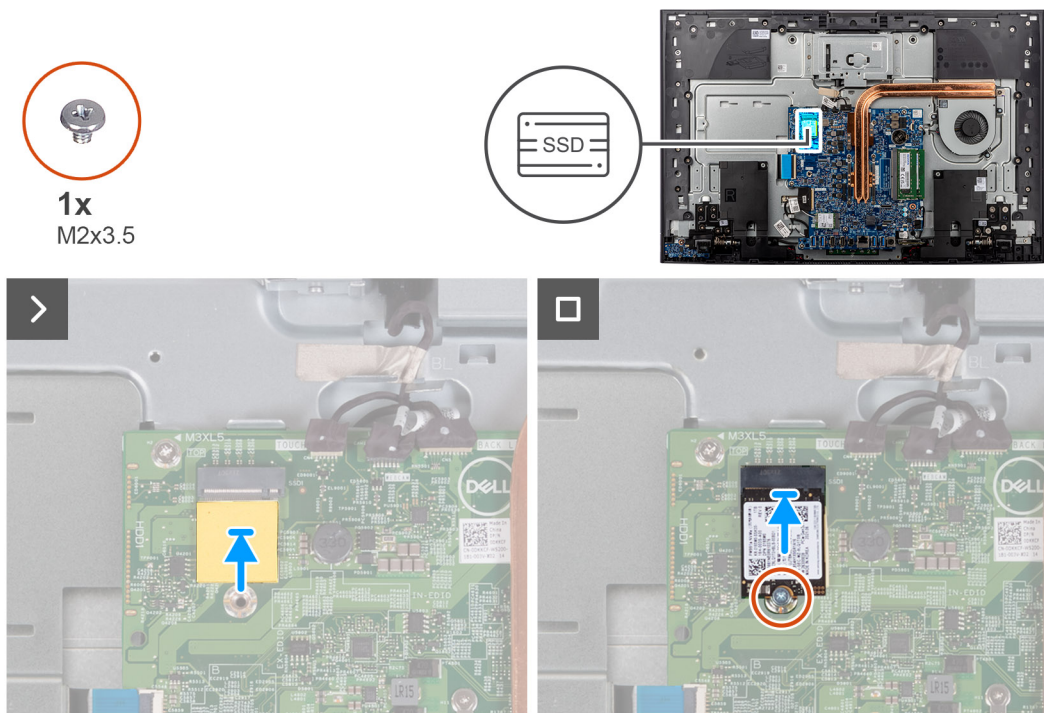
Figure 29. Installing the M.2 2230 solid-state drive
