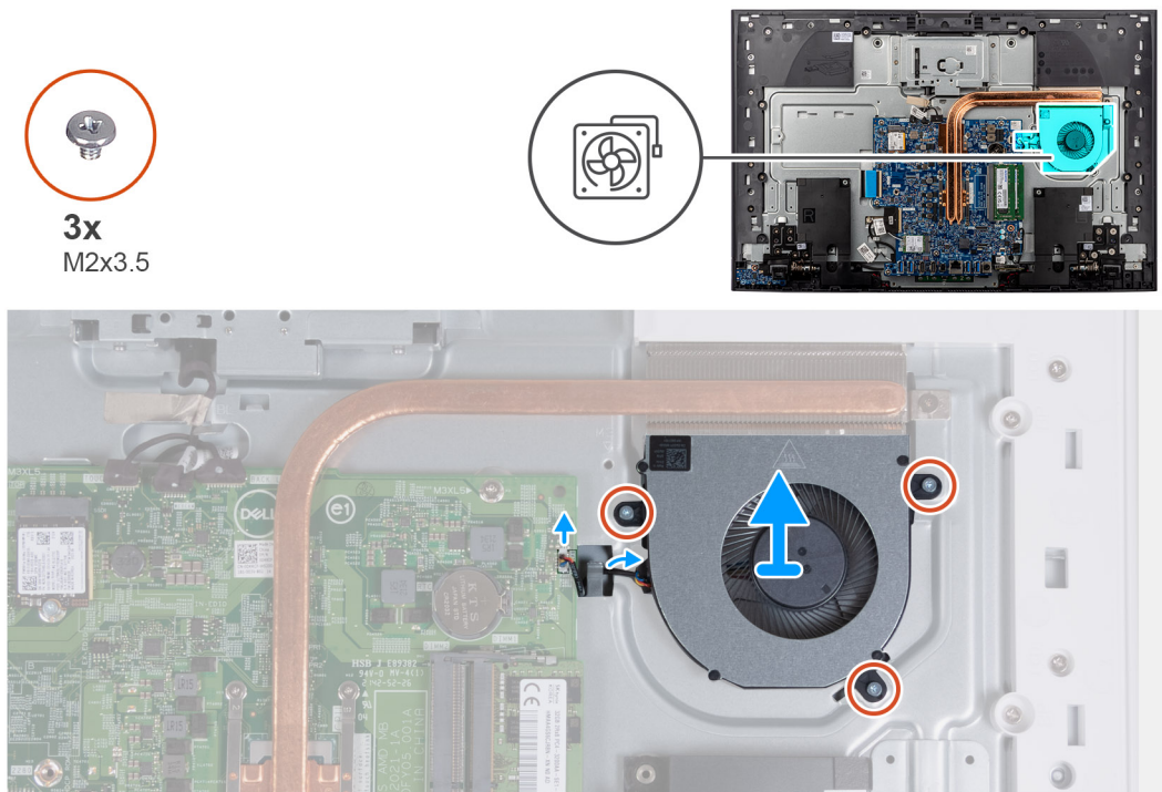
Figure 36. Removing the fan
