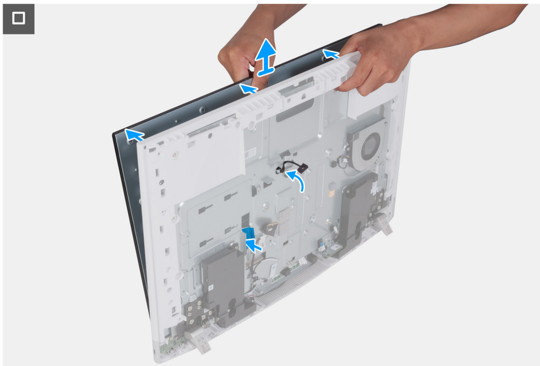
Figure 61. Removing the display panel
