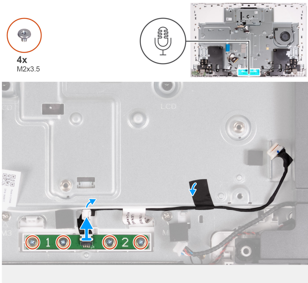
Figure 56. Removing the microphones
