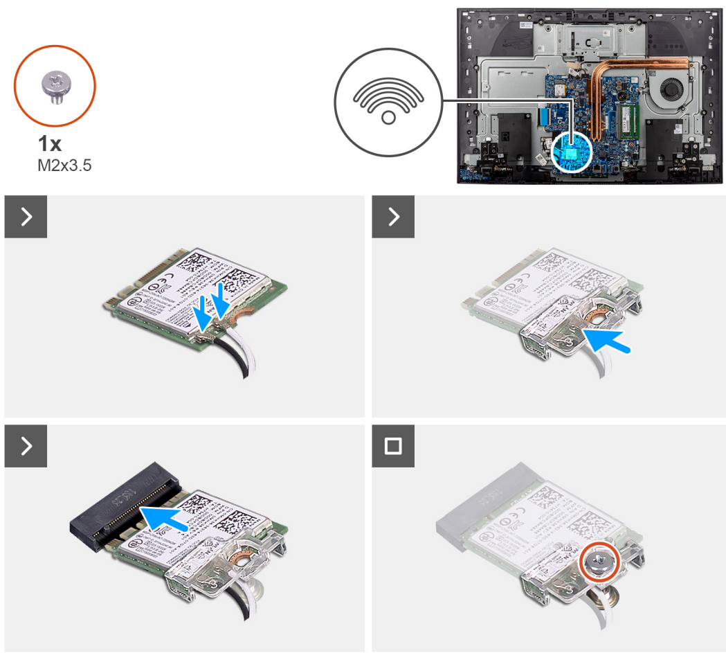
Figure 33. Installing the wireless card
