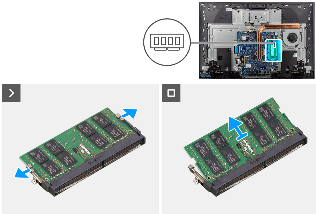
Figure 30. Removing the memory module
