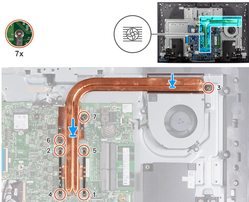
Figure 45. Installing the heat sink- discrete
