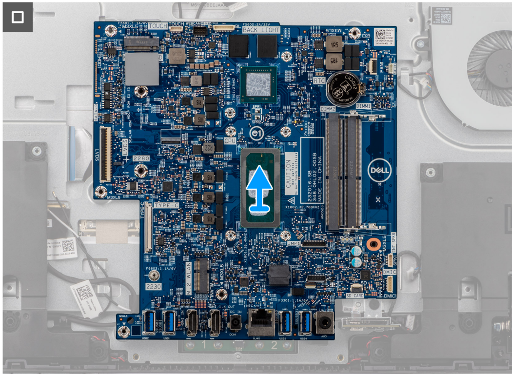
Figure 52. Lifting the system board off the chassis
