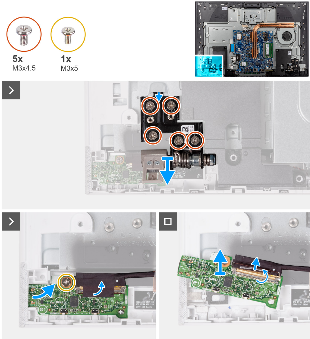
Figure 48. Removing the power-button board with USB
