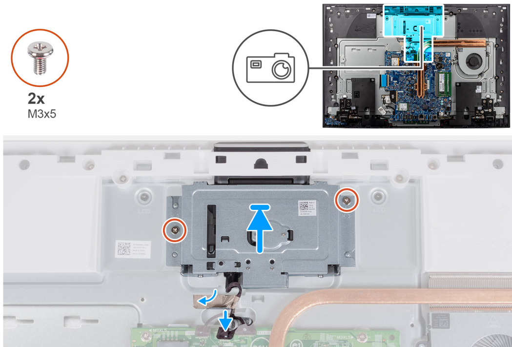
Figure 35. Installing the camera
