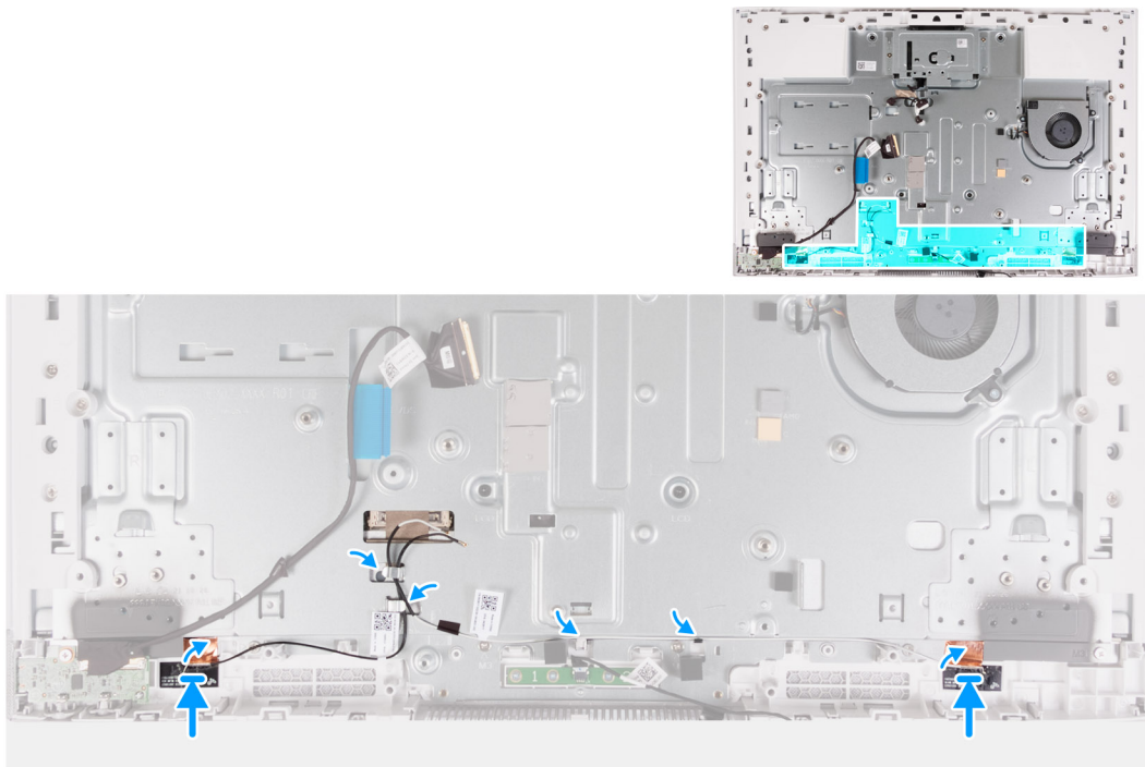
Figure 59. Installing the antennas
