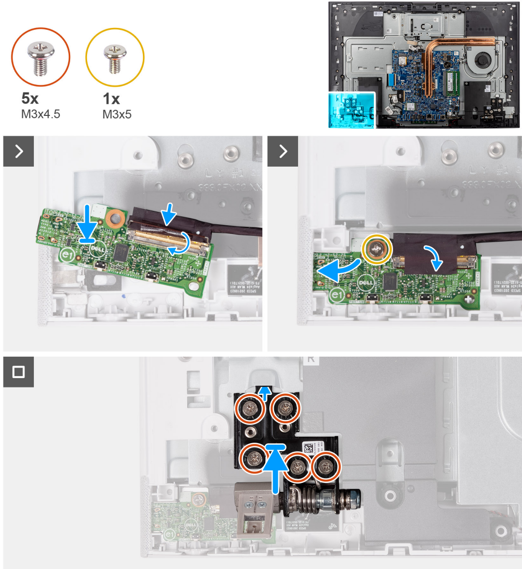
Figure 49. Installing the power-button board with USB
