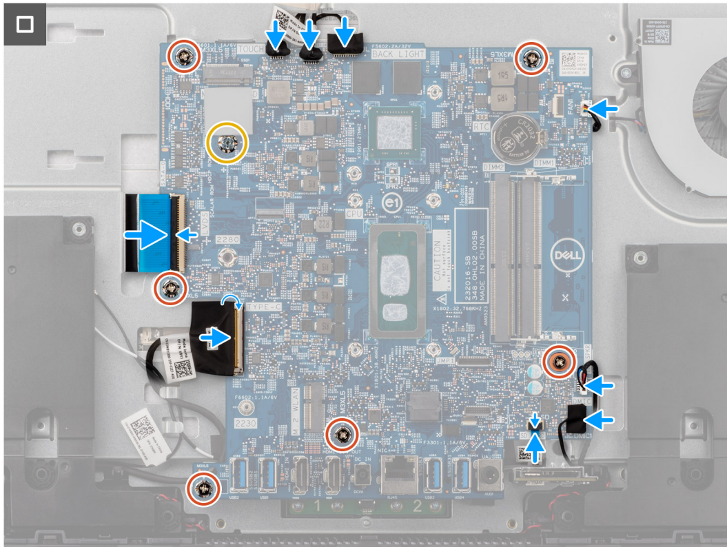
Figure 55. Installing the system board
