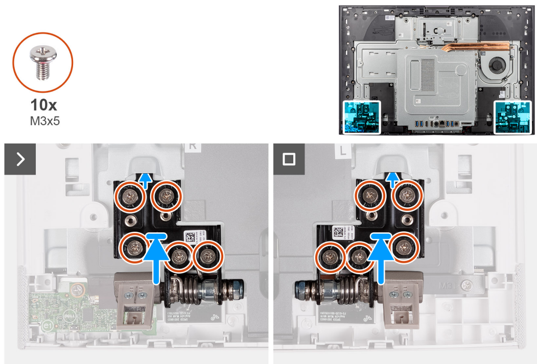
Figure 25. Installing the stand hinges
