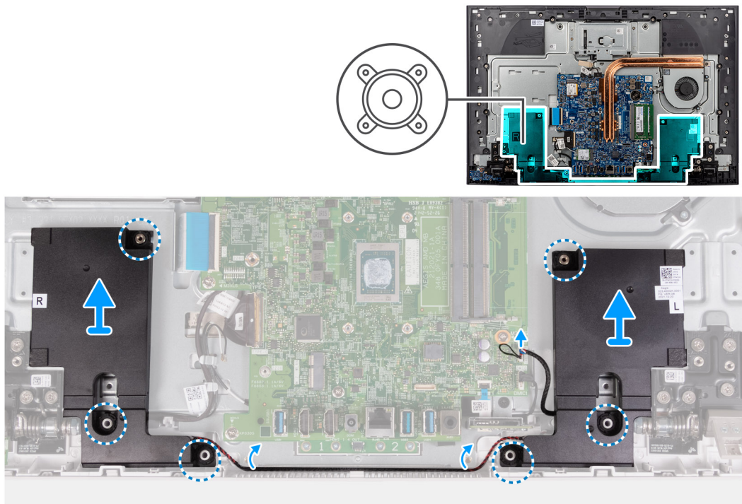
Figure 38. Removing the speakers
