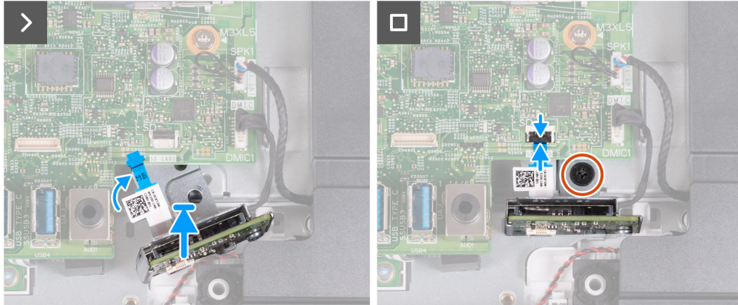
Figure 47. Installing the media-card reader
