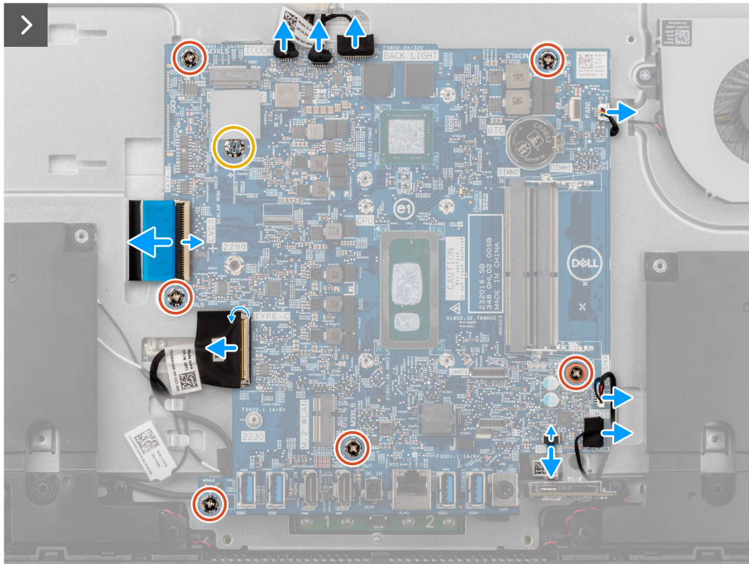
Figure 51. Removing the system board
