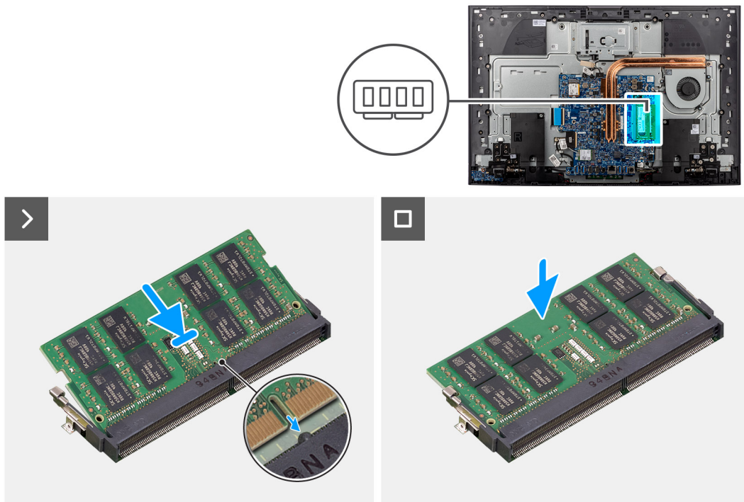
Figure 31. Installing the memory module
