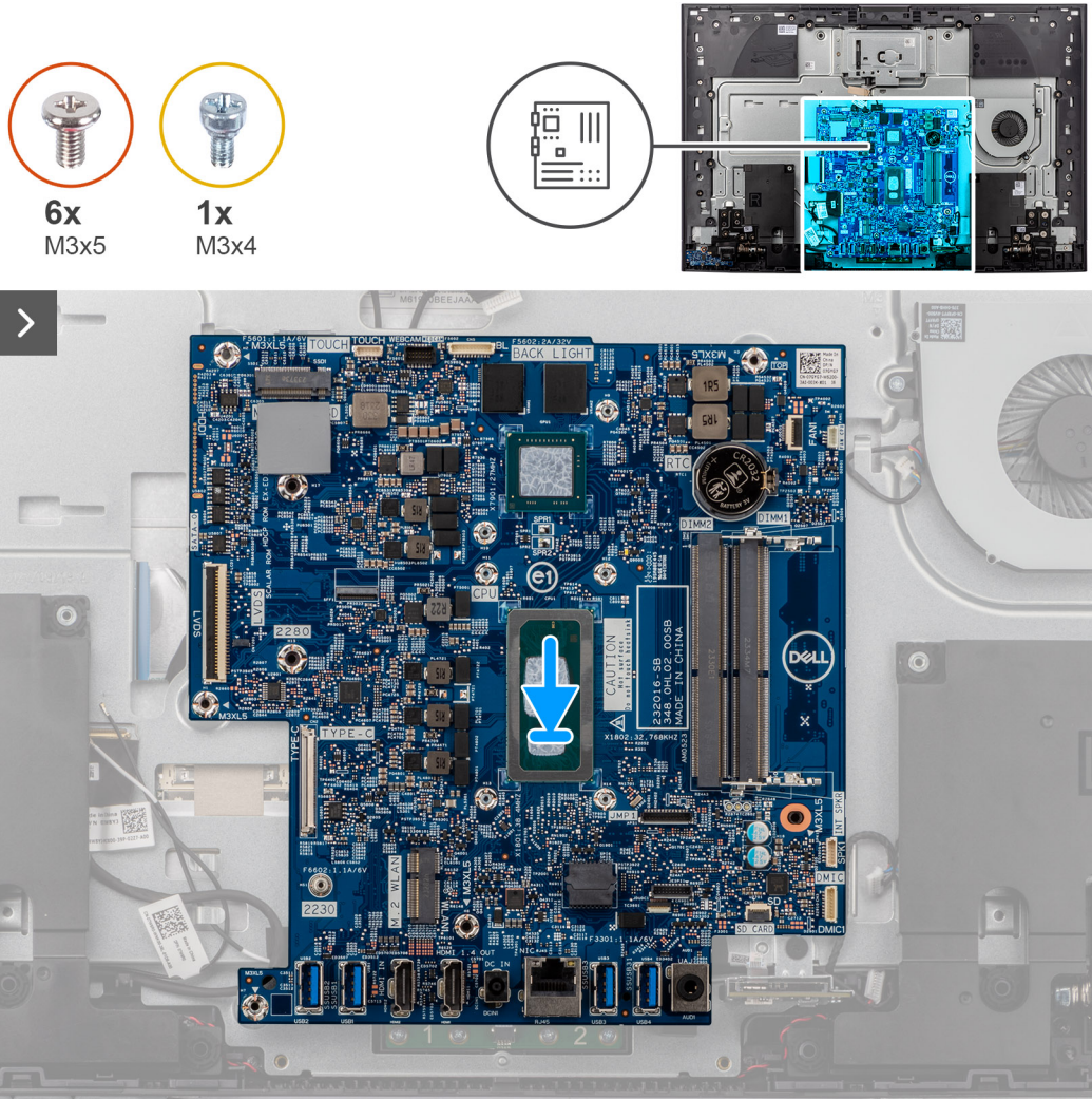
Figure 54. Placing the system board in the chassis
