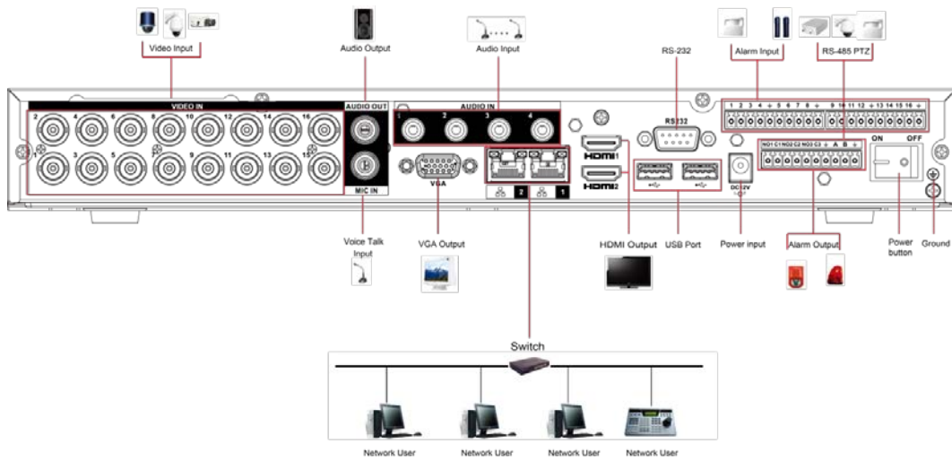
Figure 4-1 Connection diagram
