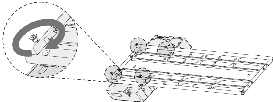
Figure 2-19 Fix HDD
