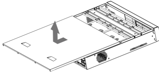
Figure 2-17 Remove cover
