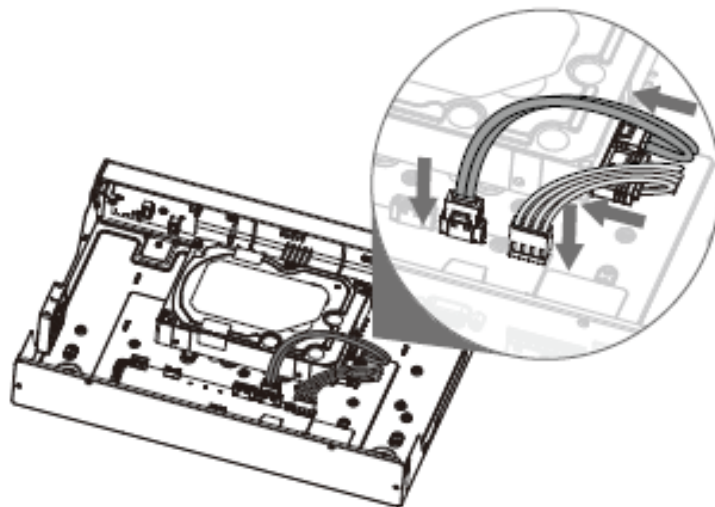
Figure 2-27 Connect cables
