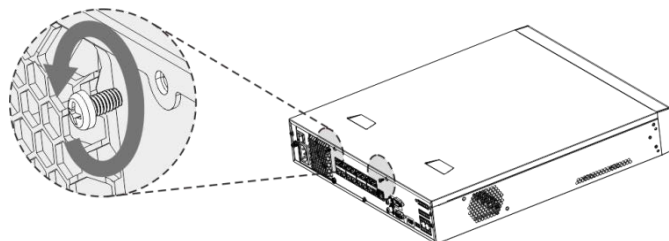
Figure 2-16 Remove screws
