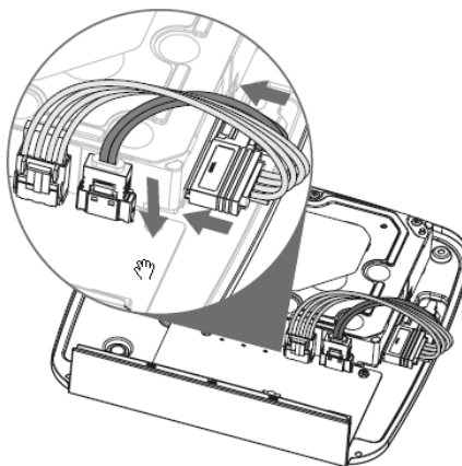
Figure 2-33 Connect cables
