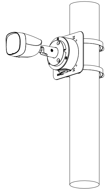
Pole Mount(Vertical)
