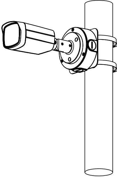
Pole Mount(Vertical)
