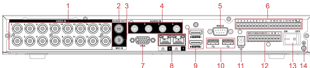
Figure 3-15 Rear panel
