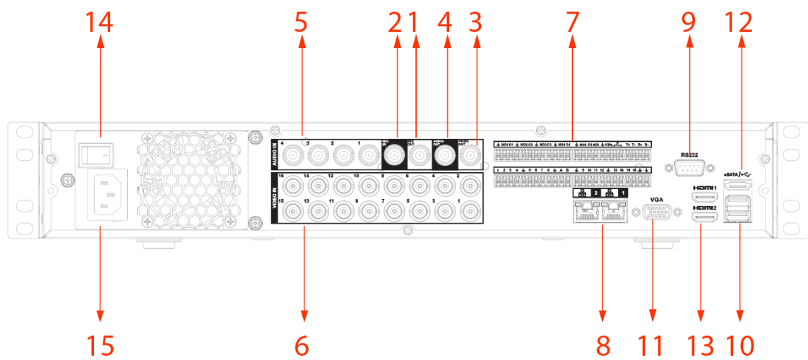
Figure 3-20 Rear panel (3)
