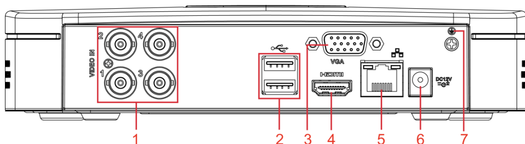
Figure 3-20 Rear panel
