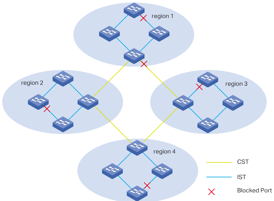
Figure 1-3 MSTP Topology
