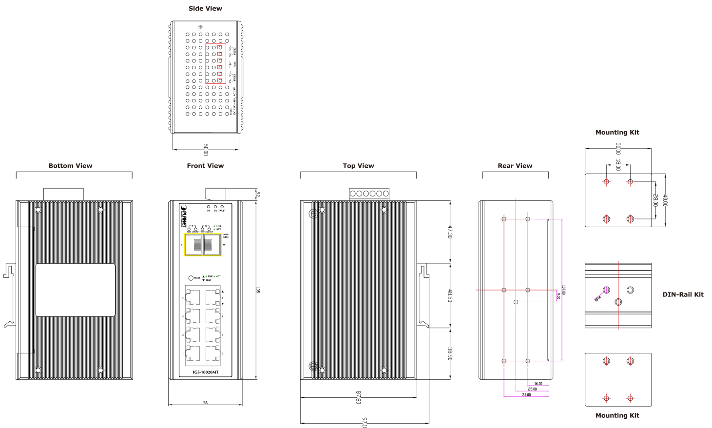
Dimensions ( unit = mm )
