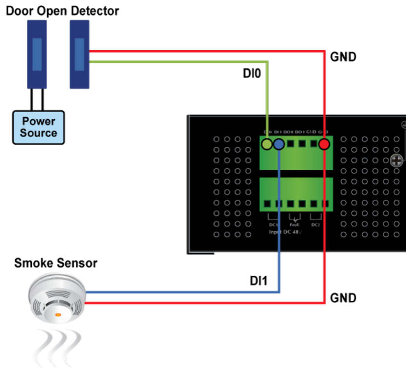
Figure 2-23 Wires DI0 and DI1 to Open Detector
