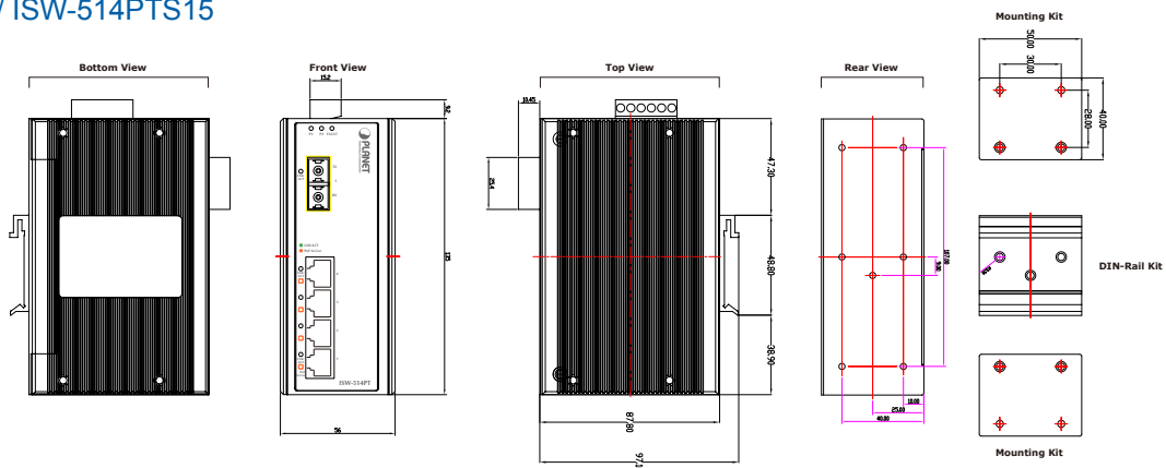
Dimensions ( unit = mm )
