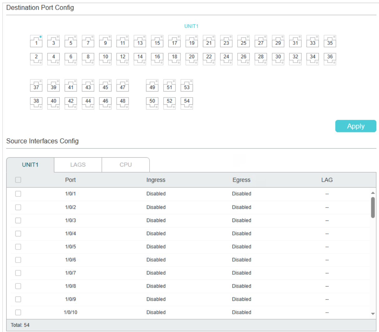
Figure 1-2 Configure the Mirroring Session
