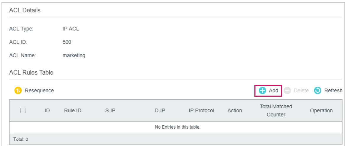
Figure 3-15 Editing IP AC
