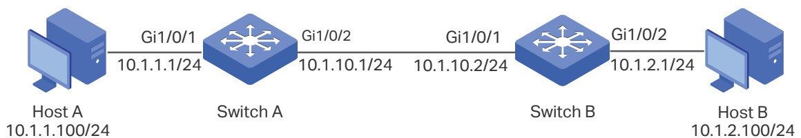
Figure 9-1 Network Topology
