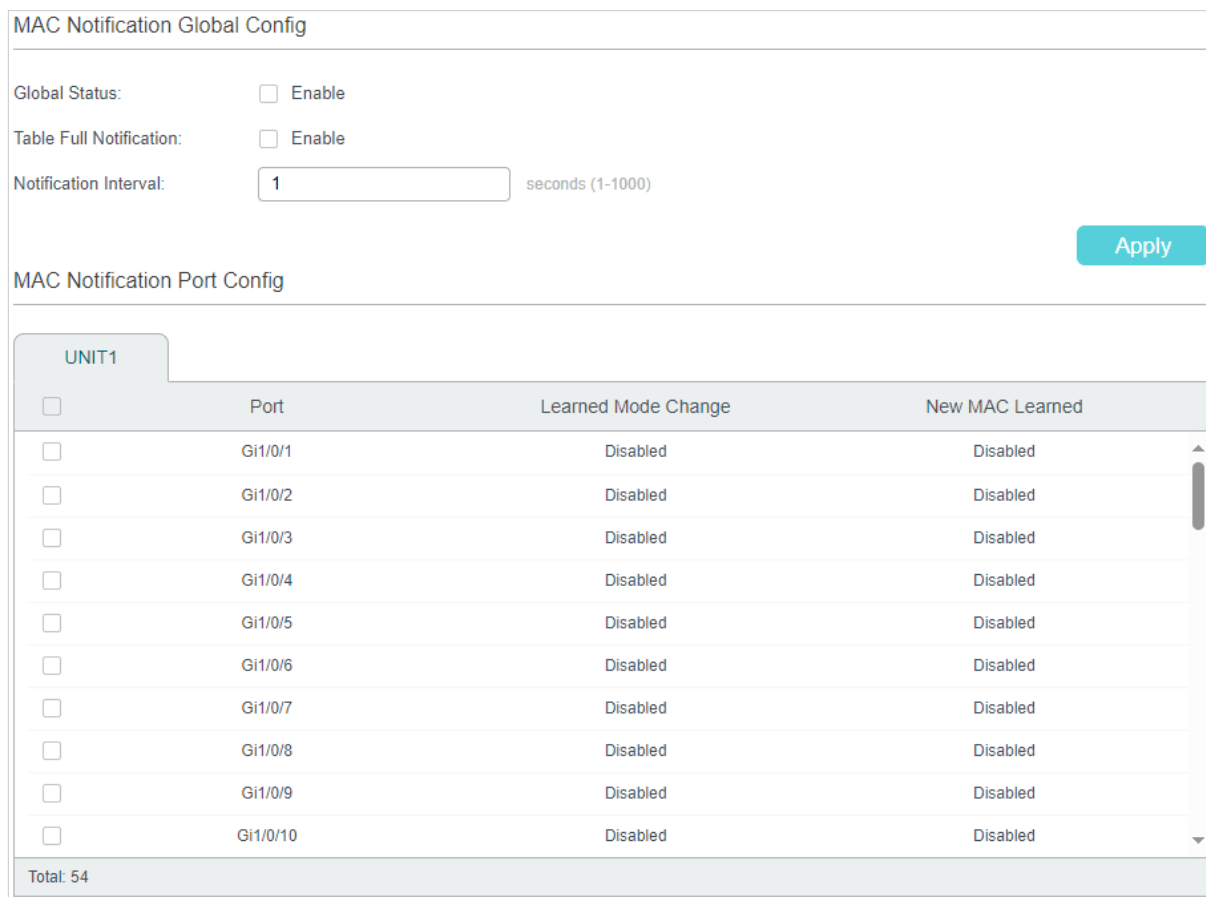
Figure 3-1 Configuring MAC Notification Traps
