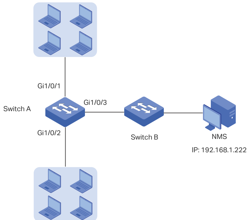
Figure 6-1 Network Topology
