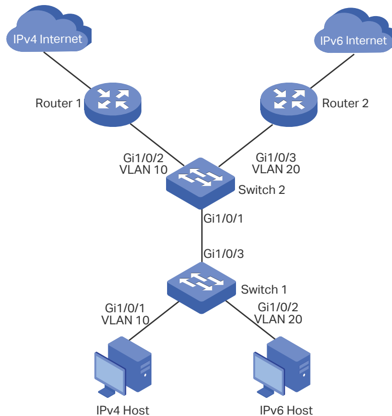
Figure 3-1 Network Topology
